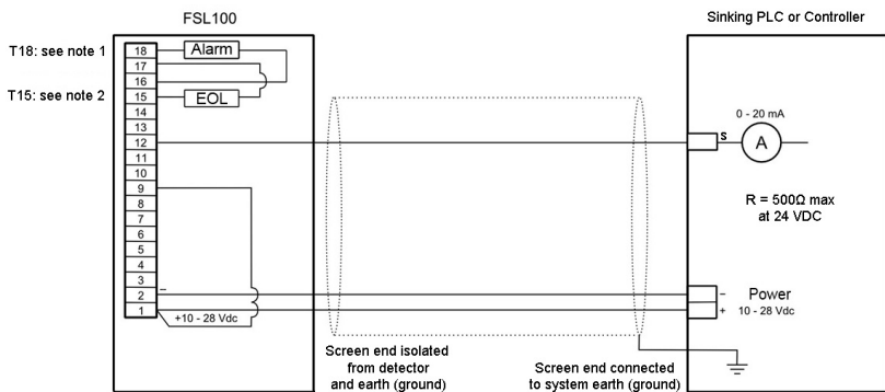
Figure 5. Wiring to a PLC or controller with a 4-20 mA sinking input
