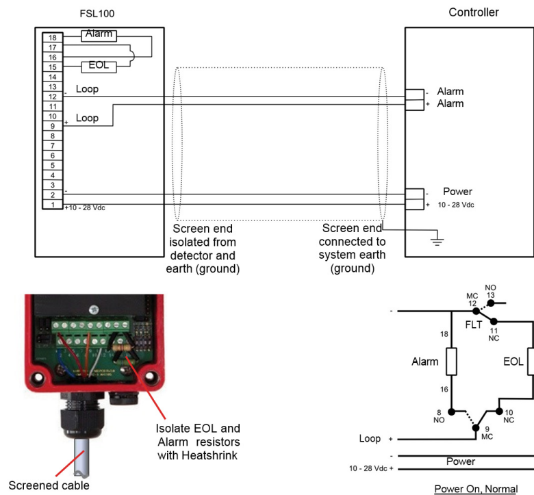
Figure 3. Control panel wiring
