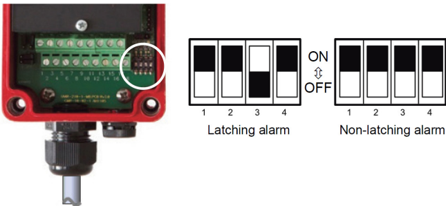
Figure 6. Latching alarm settings
