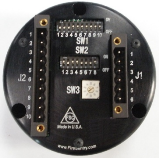
Figure 2-10 Detector Module “puck” (rear view)
