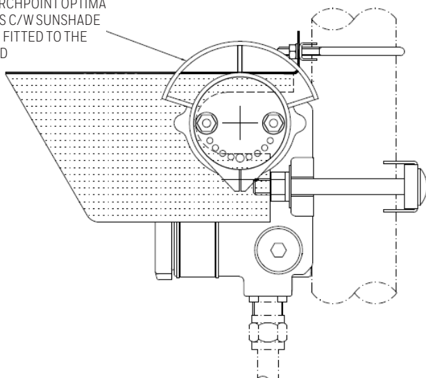
<Figure 4. OELD with Sunshade>
