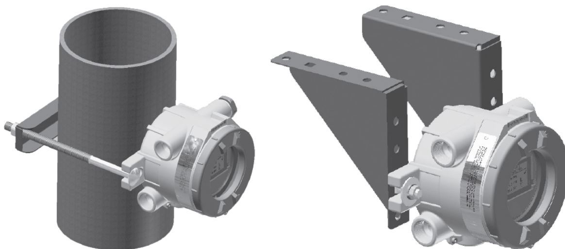
<Figure 6. Pipe and Ceiling Mount Installation Examples>
